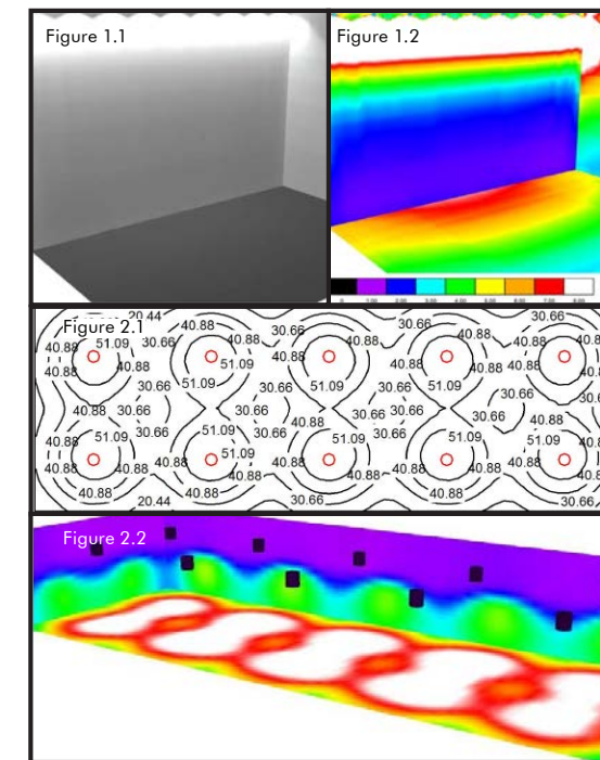
Fig 1: Simulation of Arani Floodlights in a Theatre 1.1: 3D Rendering 1.2: False Color Rendering
