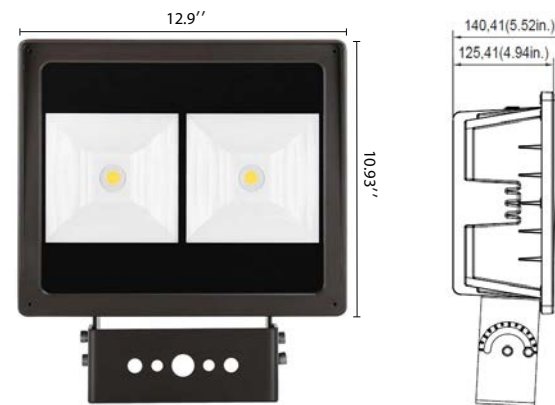
110W High Lumen Flood Light (Bracket) FL-110W-xxK-V2
