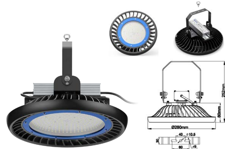
LED High Bay HB-xxxW-xxK-DS
