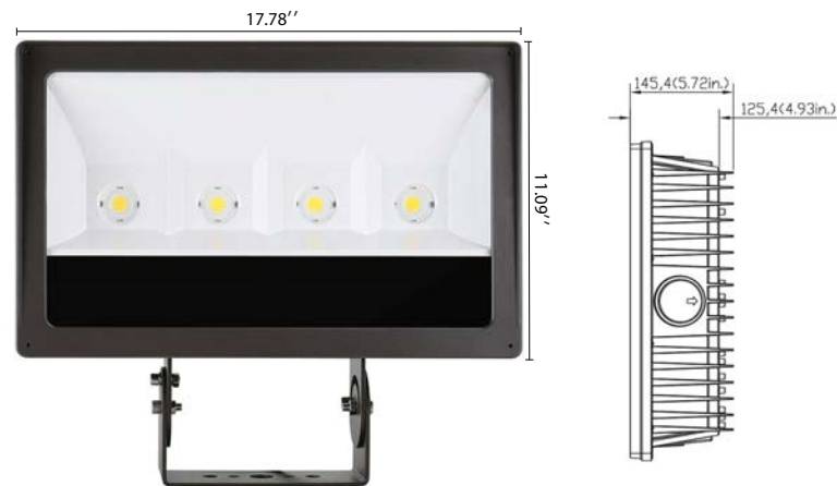
140W High Lumen Flood Light (Bracket) FL-140W-xxK-V2
