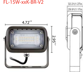
15W High Lumen Flood Light (Bracket) FL-15W-xxK-BR-V2
