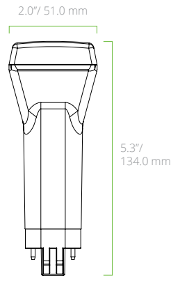
L5.5W GX23 BASE VERTICAL
