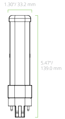
L5.5W GX23 BASE HORIZONTAL
