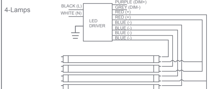
Fig.9 Single-ended Installation
