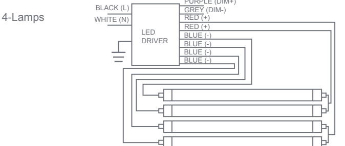
Fig.5 Double-ended Installation
