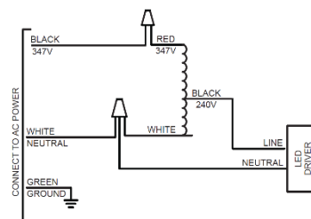
Wiring Diagram
