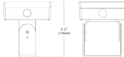
Junction Box with Trunnion Mount
