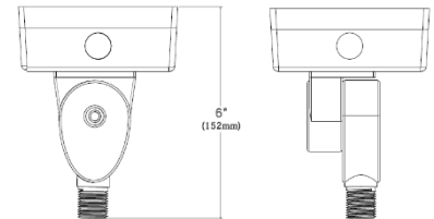
Junction Box with Knuckle Mount
