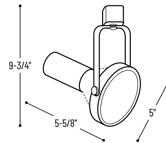
NTH-108BZ Bronze Rear Loading Gimbal
