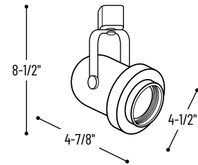
NTH-110B Black Classic Cylinder with Black Baffle
