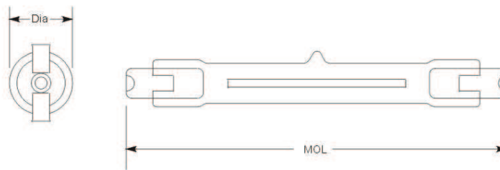
R7s Base
