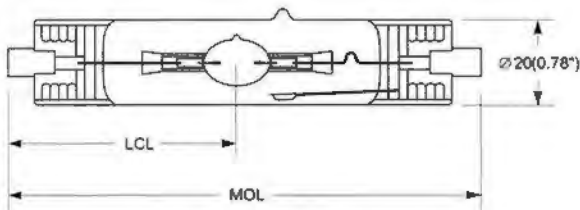
T6 Rx7s Base 70W
